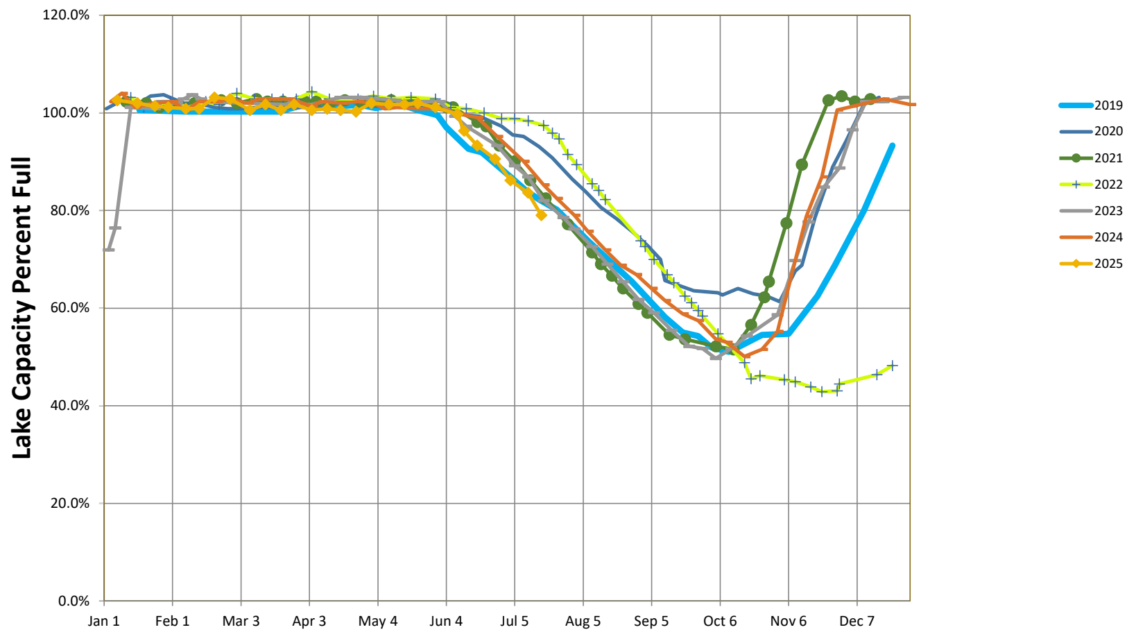
Holland Lake - Storage Volume Remaining, 2019 - 2025
