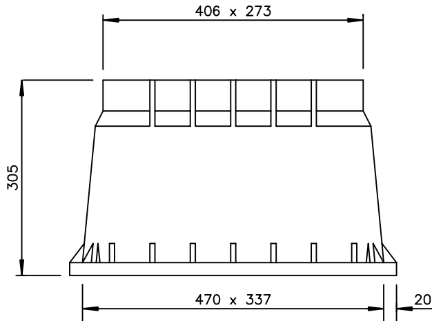
STANDARD METER BOX ELEVATION
