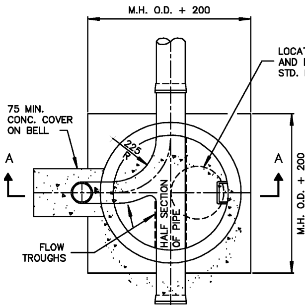
PLAN AT X-X SHOWING DROP
