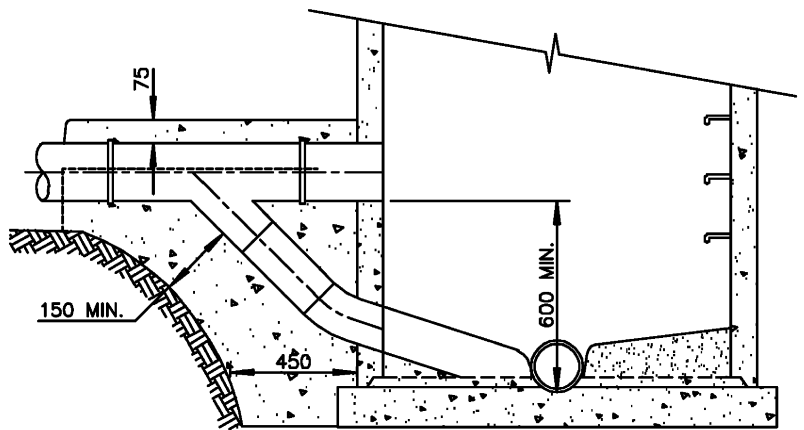
SECTION B-B DROP MANHOLE - TYPE II
