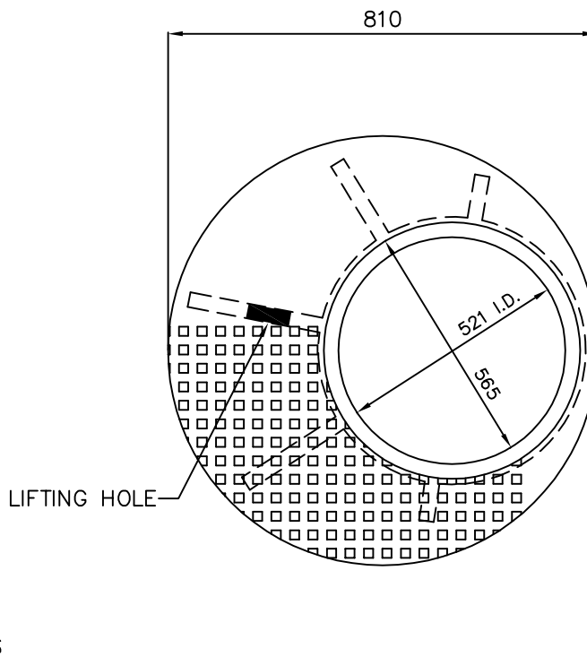
PLAN OF OUTER COVER
