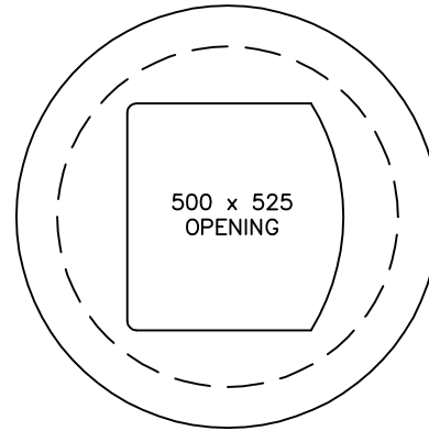
CS600 REINFORCED CONCRETE CATCH BASIN LID
