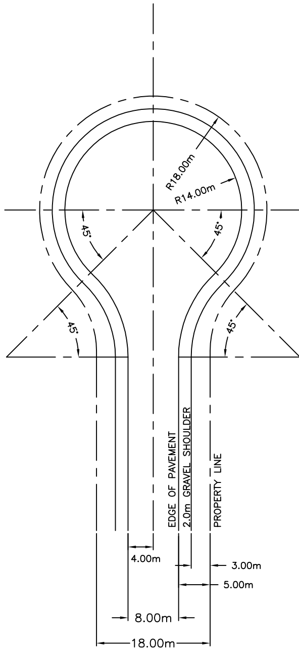
STANDARD CUL-DE-SAC
