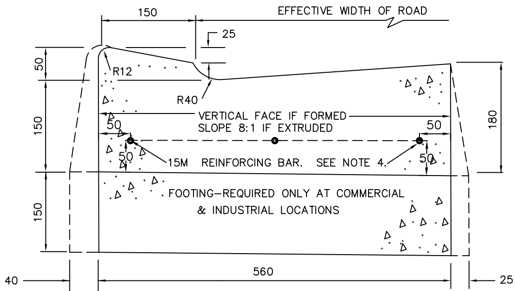
DROP CURB WITH INTEGRAL GUTTER
