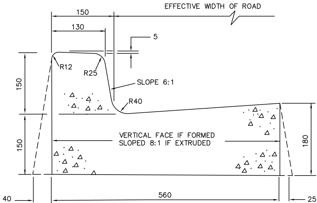
CURB WITH INTEGRAL GUTTER
