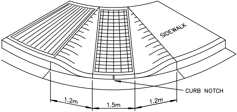
TYPE A ISOMETRIC VIEW
