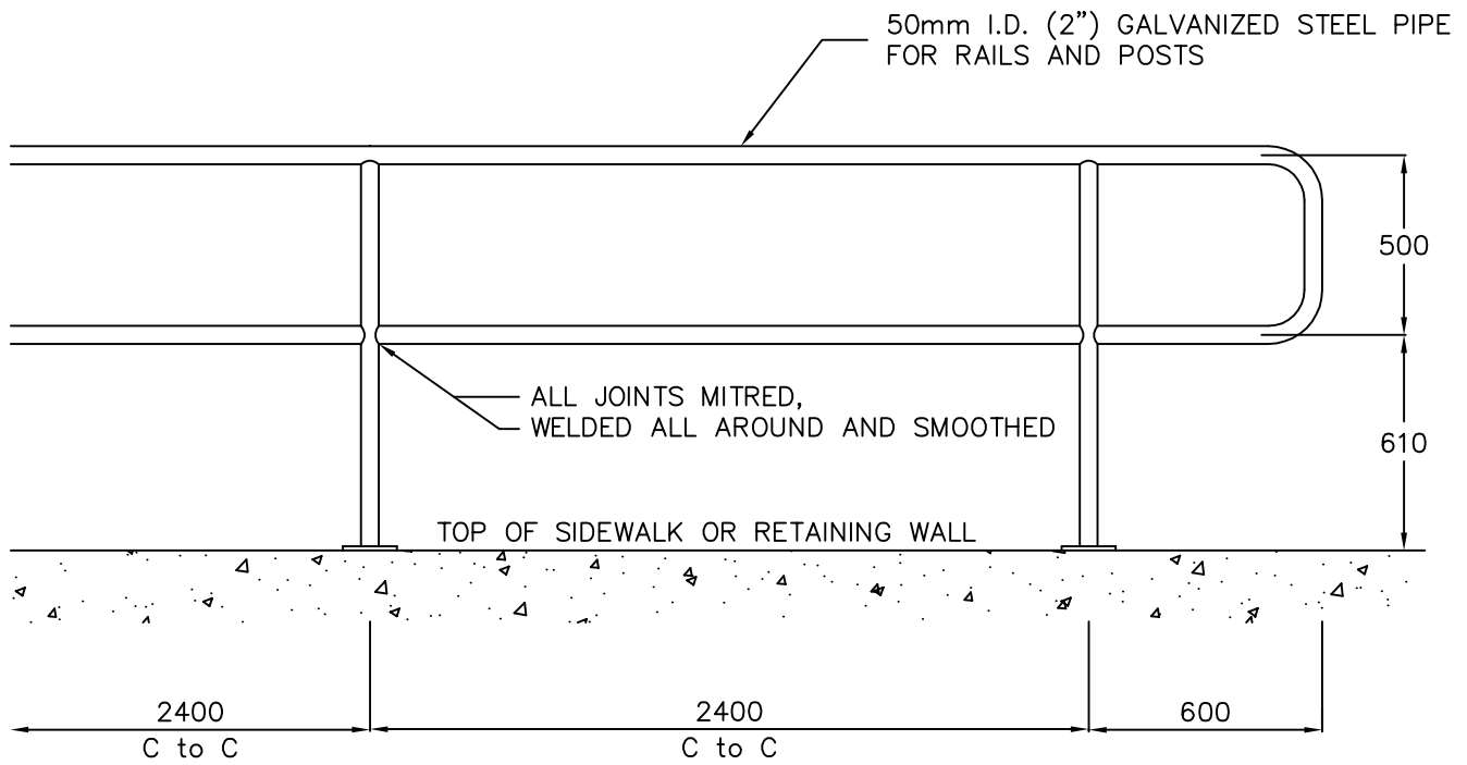
TYPICAL SIDEWALK/RETAINING WALL HANDRAIL
