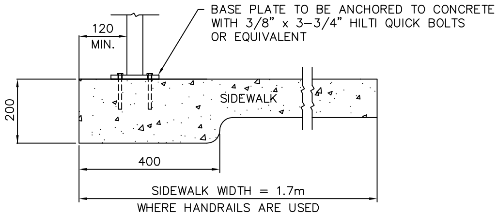
ATTACHED MOUNTING DETAIL
