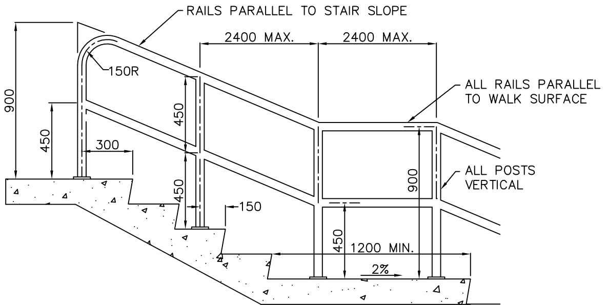
TYPICAL STAIRWAY HANDRAIL
