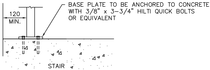
ATTACHED MOUNTING DETAIL
